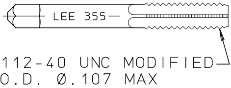
BOTTOMING TAP PLUG EXTRACTION CUTA3555503B
