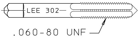
STARTER TAP PIN EXTRACTION CUTA3024403B
