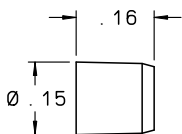
PIN
